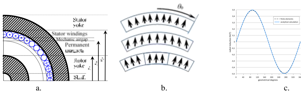
Figure 1. a. Structure of slotless machine b. Radial, radial parallel and radial parallel bars structures studied c. Normal induction waveform in airgap for a bipolar radial parallel magnetized structure.
